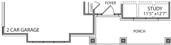
FIRST FLOOR PLAN - C
