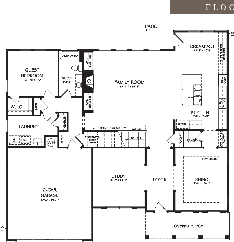
FIRST FLOOR PLAN - A
