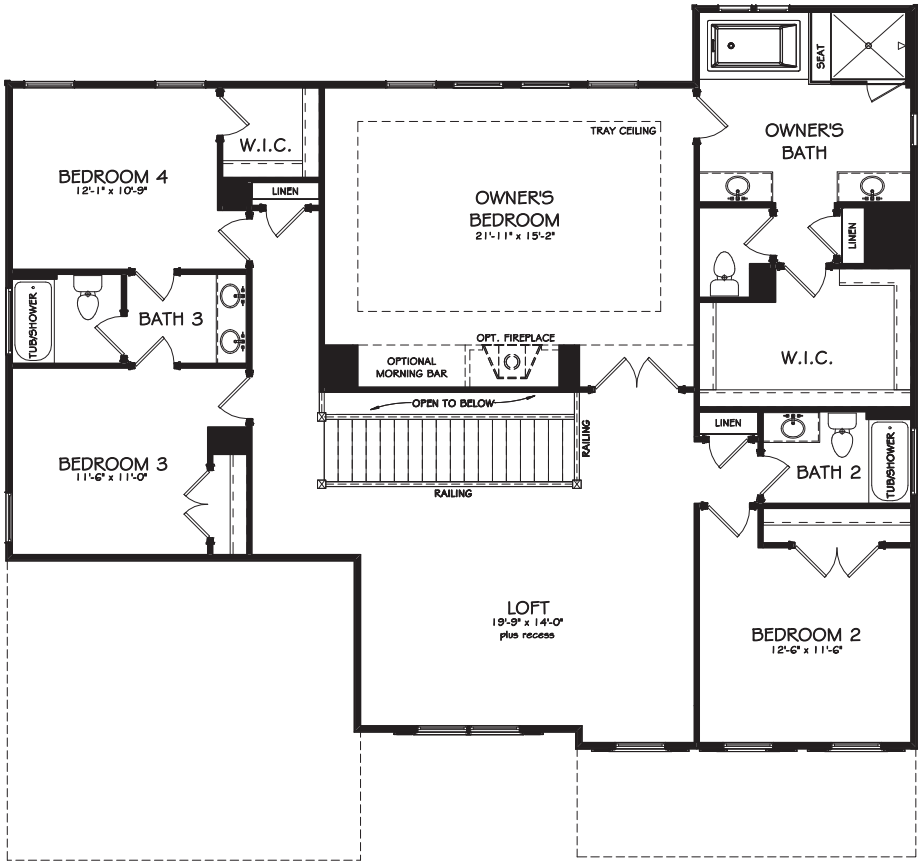
SECOND FLOOR PLAN - A
